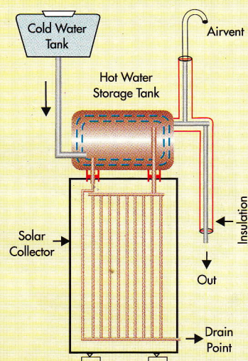
Schematic Diagram Thermosyphon System
