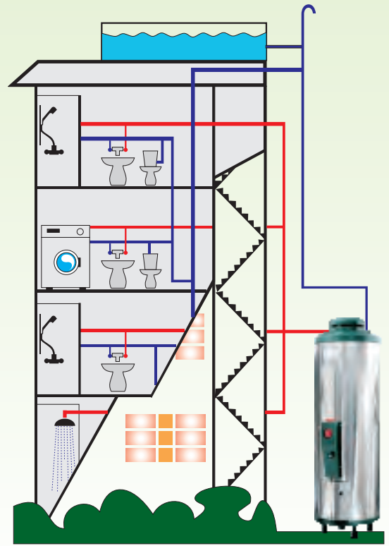
Schematic Diagram - Gravity Water Supply
